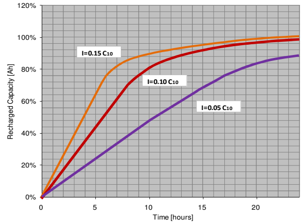
Fig. 7 : Recharge curves at 2.4 V/cell with different limit of current
