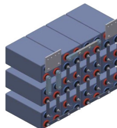
Example of installation and cell arrangement (position of + / - poles) of AGM batteries with capacity equal or higher than 800Ah
