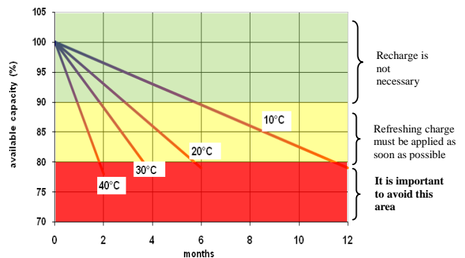
Fig. 8 : Storage time versus temperatures
